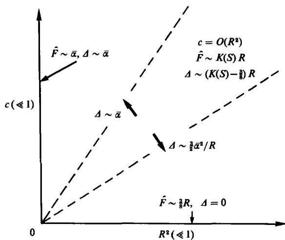
FIGURE 2. Dependence of \Delta and \tilde{F} on R and c . Here S = \bar{\alpha}^2/R^2 and \bar{\alpha}^2 \sim \frac{3}{8}c .
