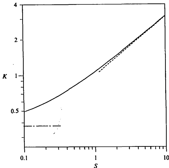
FIGURE 1. Log-log plot of K given by (3.13) vs. S \sim \frac{3}{8}c/R^2 (—). K = S^{\frac{1}{2}} (---) and K = \frac{3}{8} (-·-·-) are also plotted.
